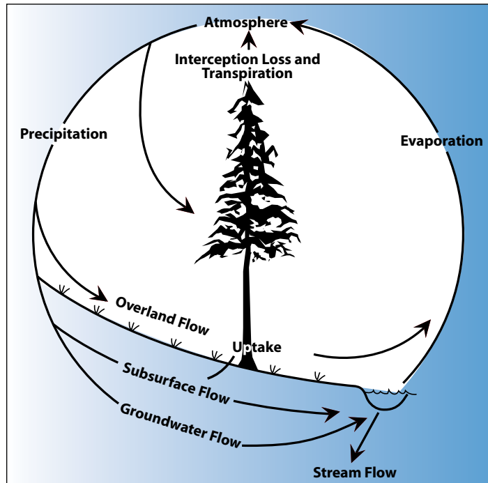
Figure 4. Forest hydrologic cycle.
